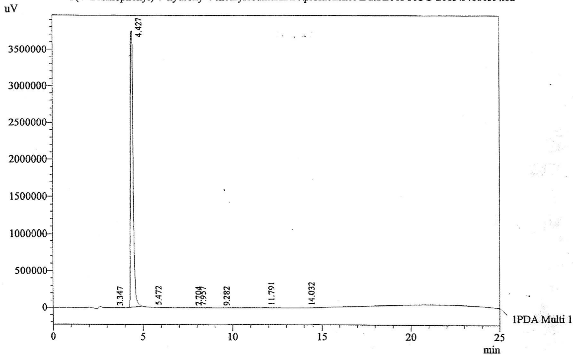
Chromatogram 3(4'-Bromophenyl)-7-hydroxy-4-methylcoumarin D:\promonence\Data\2013\AUG-2013\140813F.lcd
